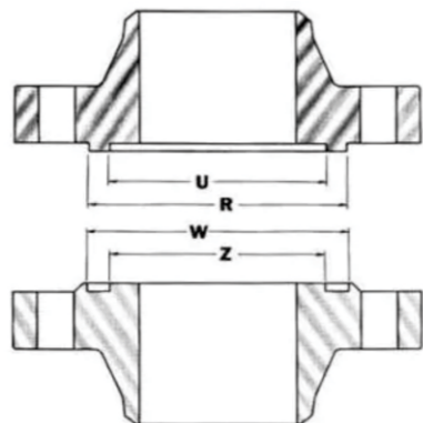
Large-Tongue-and-Groove
