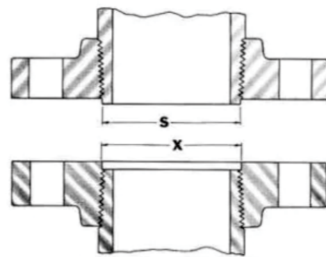
Small-Male-and-Female on-end-of-pipe
