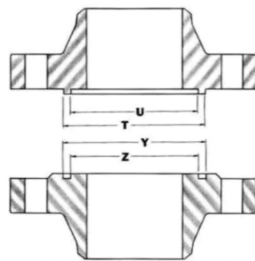
Small-Tongue-and-Groove
